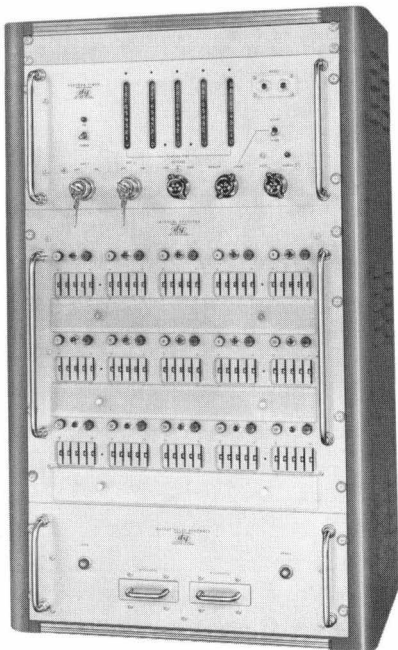
Typical of special instrumentation produced by -hp- 's Dymec division is above program timing system. System will start and/or stop 15 external functions in a programmable sequence by contact closures. System used for such purposes as controlling critical phases of missile test runs and firings. Accuracy is derived from internal crystal time base.
