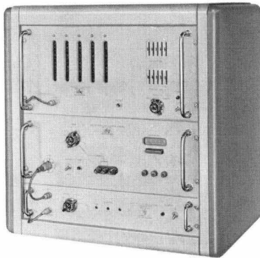
Dymec go-no go measuring set measures and compares dc voltages against preset limits, then provides go-no go output signals. System also makes results available for recording by digital recorder. Measurement accuracy is \pm 0.1\% .
