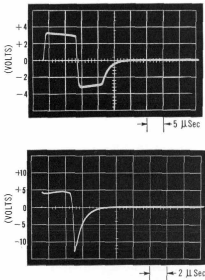
Fig. 8. Detail of output pulses provided by Model 2210 (upper) and Model 2211 (lower) voltage-to-frequency converters.
