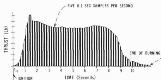
Fig. 2. Above time-plot of rocket thrust typifies data-measuring and logging abilities of equipment in Fig. 1 when used with digital printer (see Fig. 3). Equipment arrangement is simple, fast, and has low susceptibility to noise.
