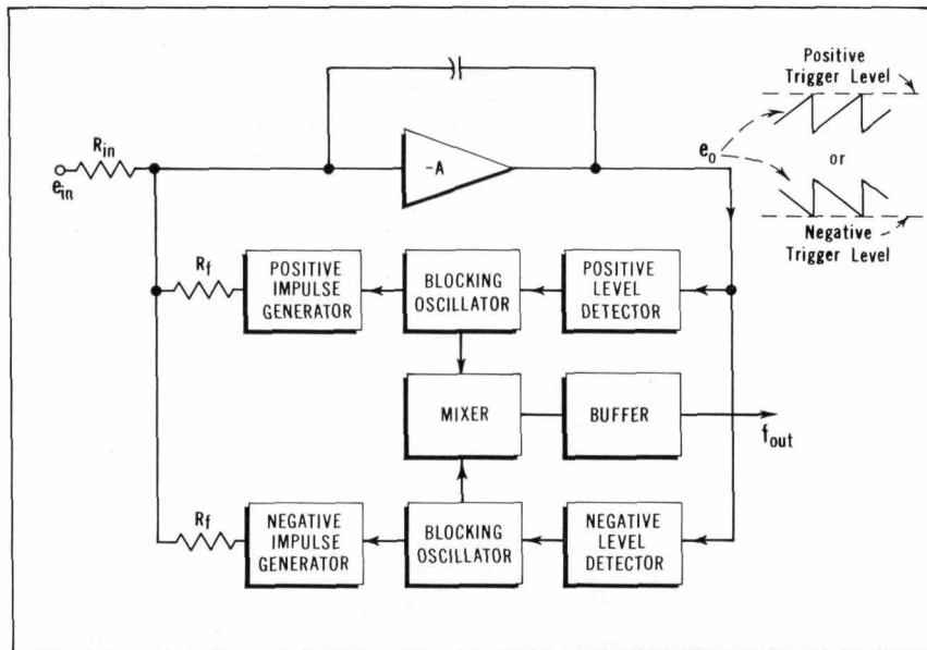
Fig. 5. Basic circuit arrangement of voltage-to-frequency converter. Circuit uses true analog integrator in generating output pulses whose frequency is proportional to integral of voltage being measured.
