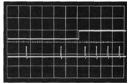
Fig. 9. Oscillogram illustrating how converter output frequency responds to a fast input voltage change from one level to another at same polarity. Converter produces new pulse of proper rate within one period of new frequency. Because of averaging effect of converter and counter, the counted output pulses accurately include a fast change in input such as this.
