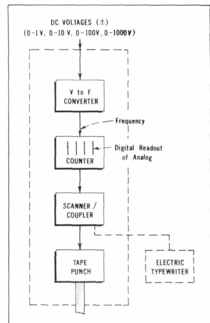
Fig. 4. Converter and counter combination can be used to measure and record data on punched tape or electric typewriter. Four- or five-digit resolution can be obtained at an accuracy of better than 0.1%.
