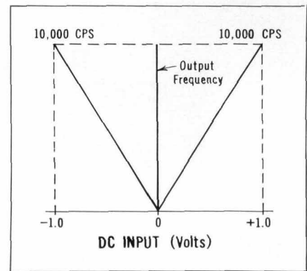
Fig. 6. Input voltage-output frequency characteristic of basic Dymec voltage-to-frequency converter. Models producing 100 kc full scale are also available.
