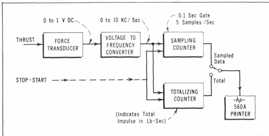
Fig. 3. Equipment arrangement used to log rocket-thrust data plotted in Fig. 2. Besides measuring and logging samples at rate of several per second, equipment also totalizes overall measurement.
